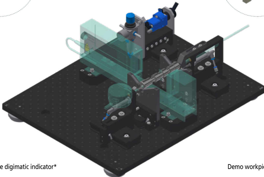
K551595 Shaft Measuring Kit Mitutoyo Basic*
